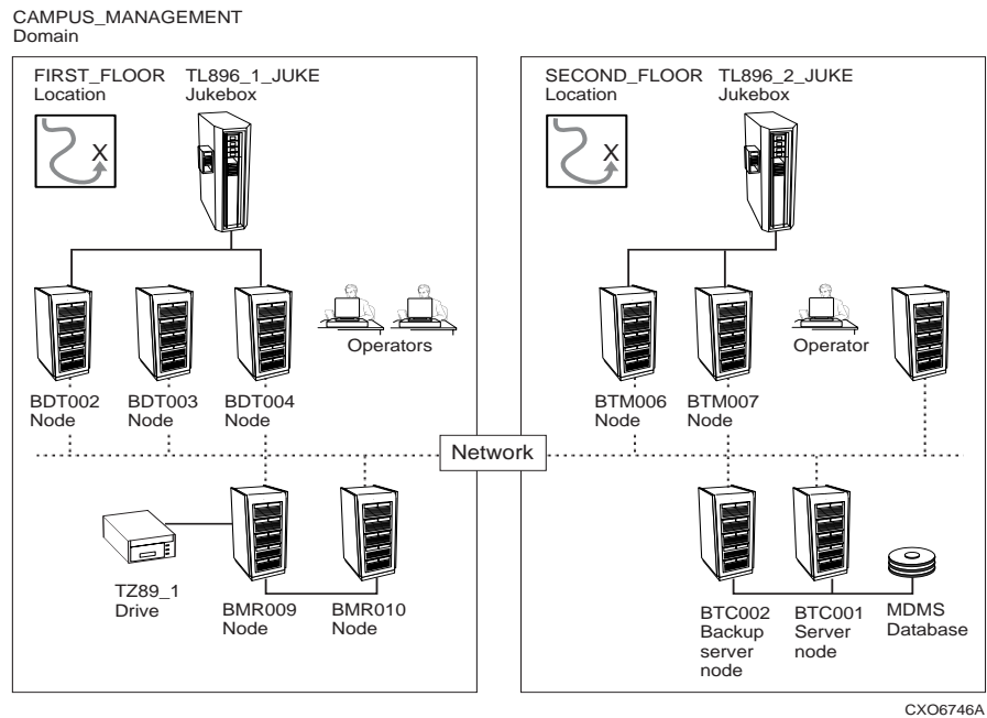
Figure 11–1 The MDMS Domain
