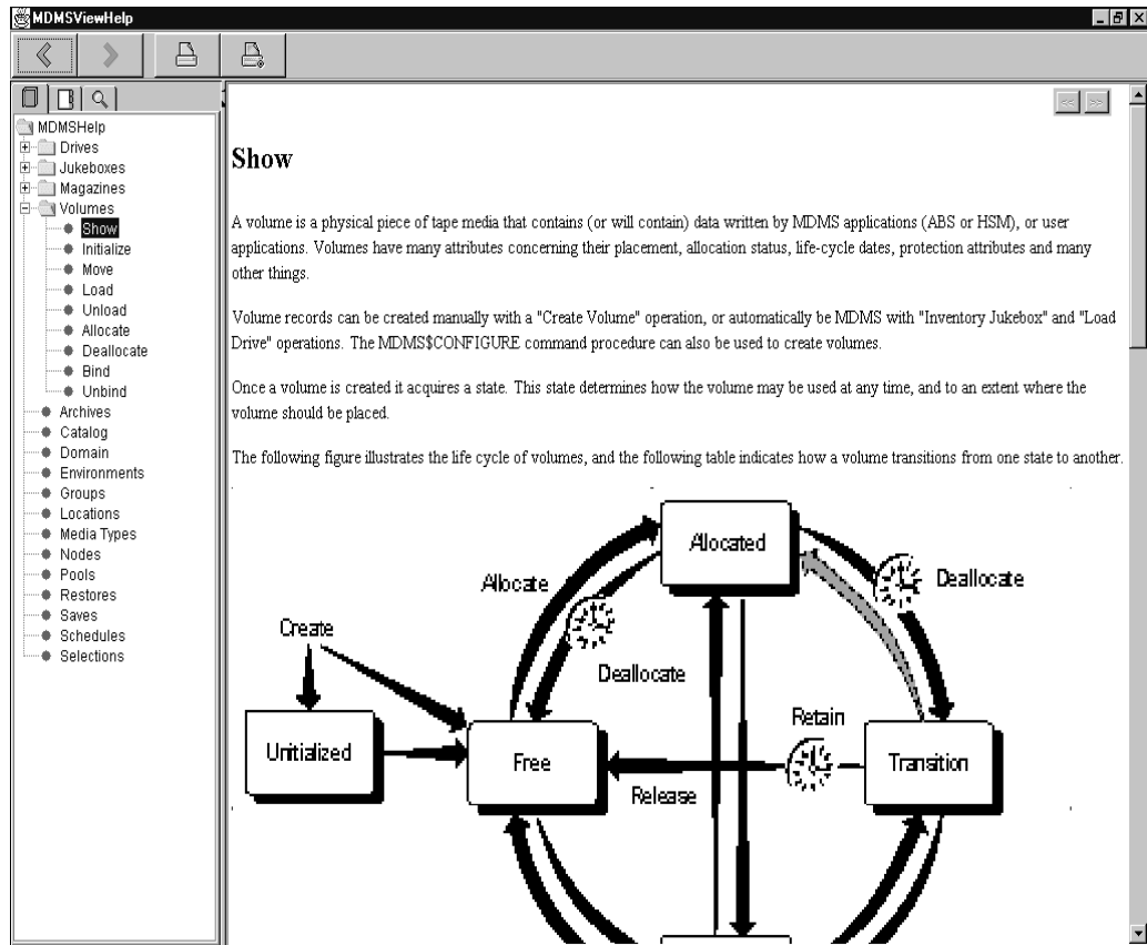
Figure 9–9 Context-Sensitive Help Screen from Show Volume Screen
