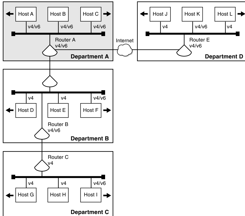
Figure 9–5: Routing IPv6 Traffic from Host A to Host K
