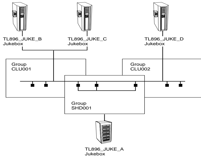
Figure 11–2 Groups in the MDMS Domain
